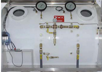
Plumbed Chamber
